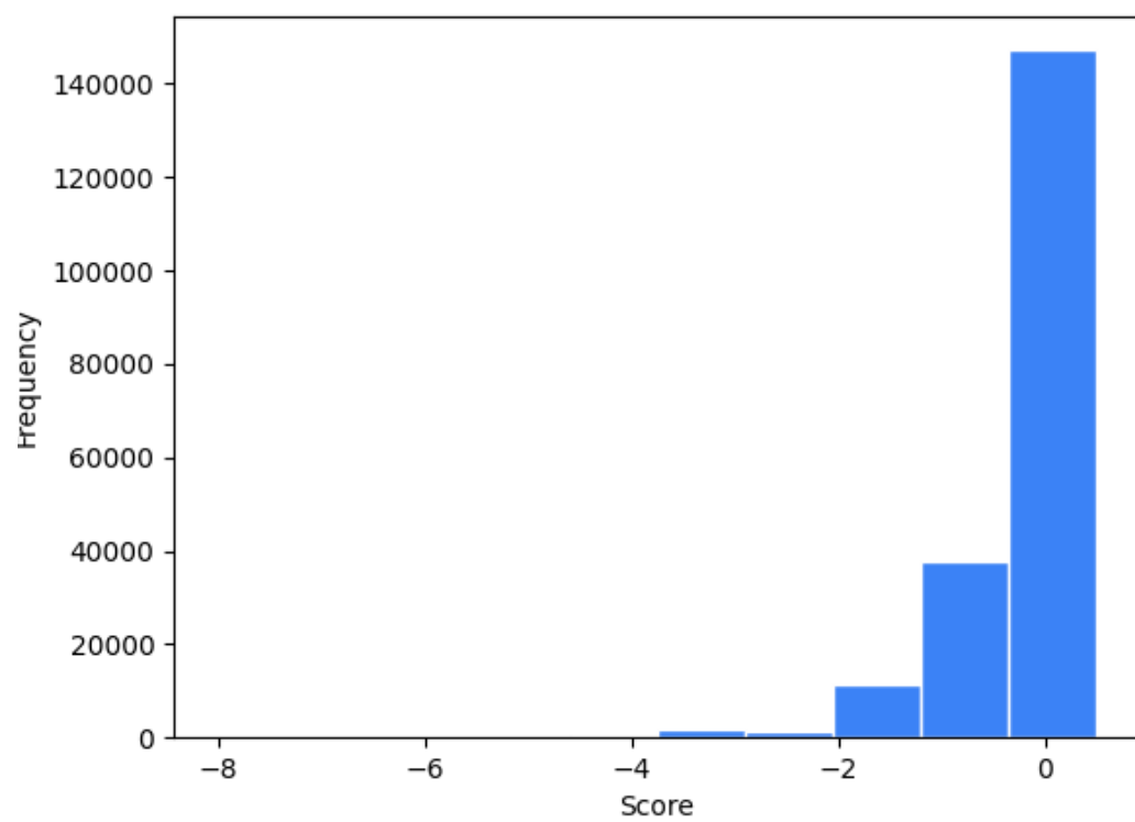
Score Distribution
